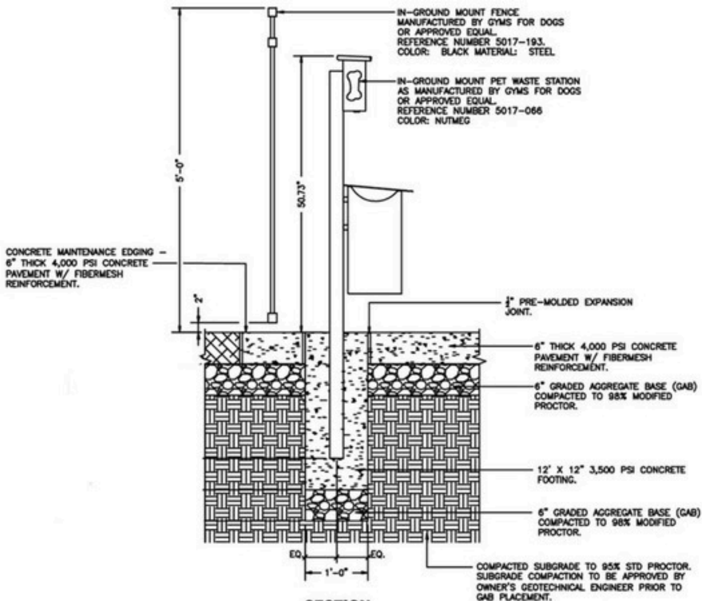
SECTION
