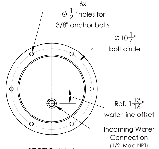
SECTION A-A Flange Hole Pattern
